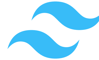
TailwindCSS
