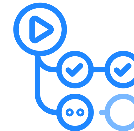
Github Actions
