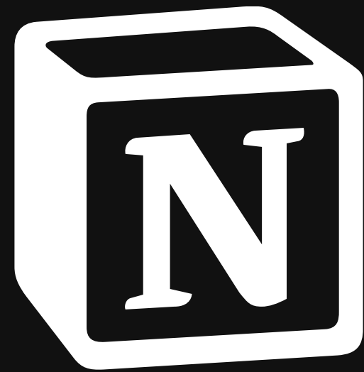
Notion
