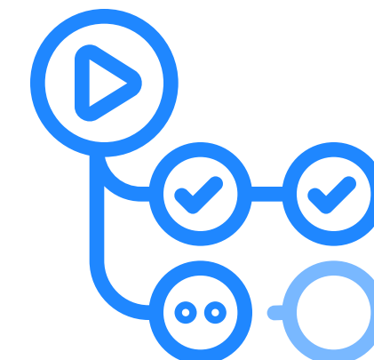
Github Actions
