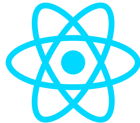
React
